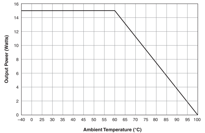
Output Power vs. Ambient Temperature V_{IN} = Nominal, Natural Convection
