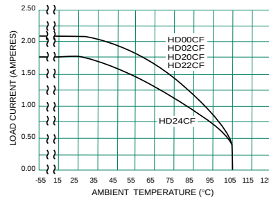
LOAD CURRENT DERATING CURVE FIGURE 3
