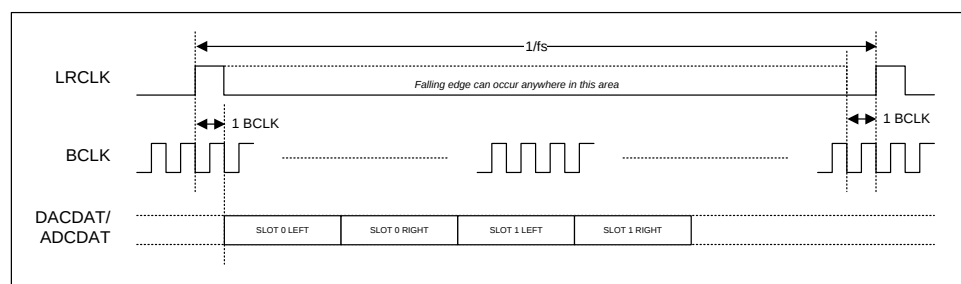
Figure 60 TDM in DSP Mode A
