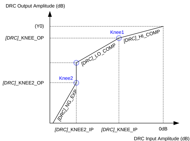
Figure 24 DRC Response Characteristic
