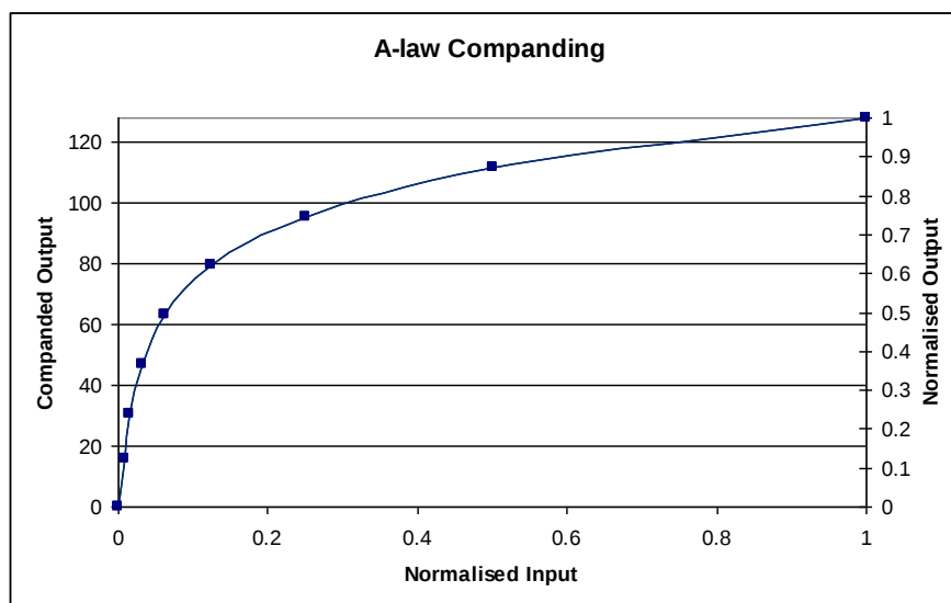
Figure 64 A-Law Companding
