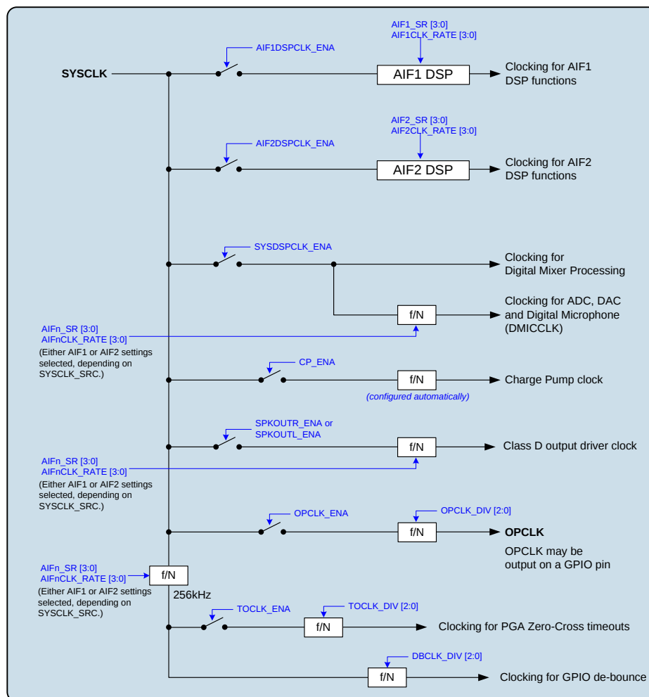
Figure 68 System Clocking
