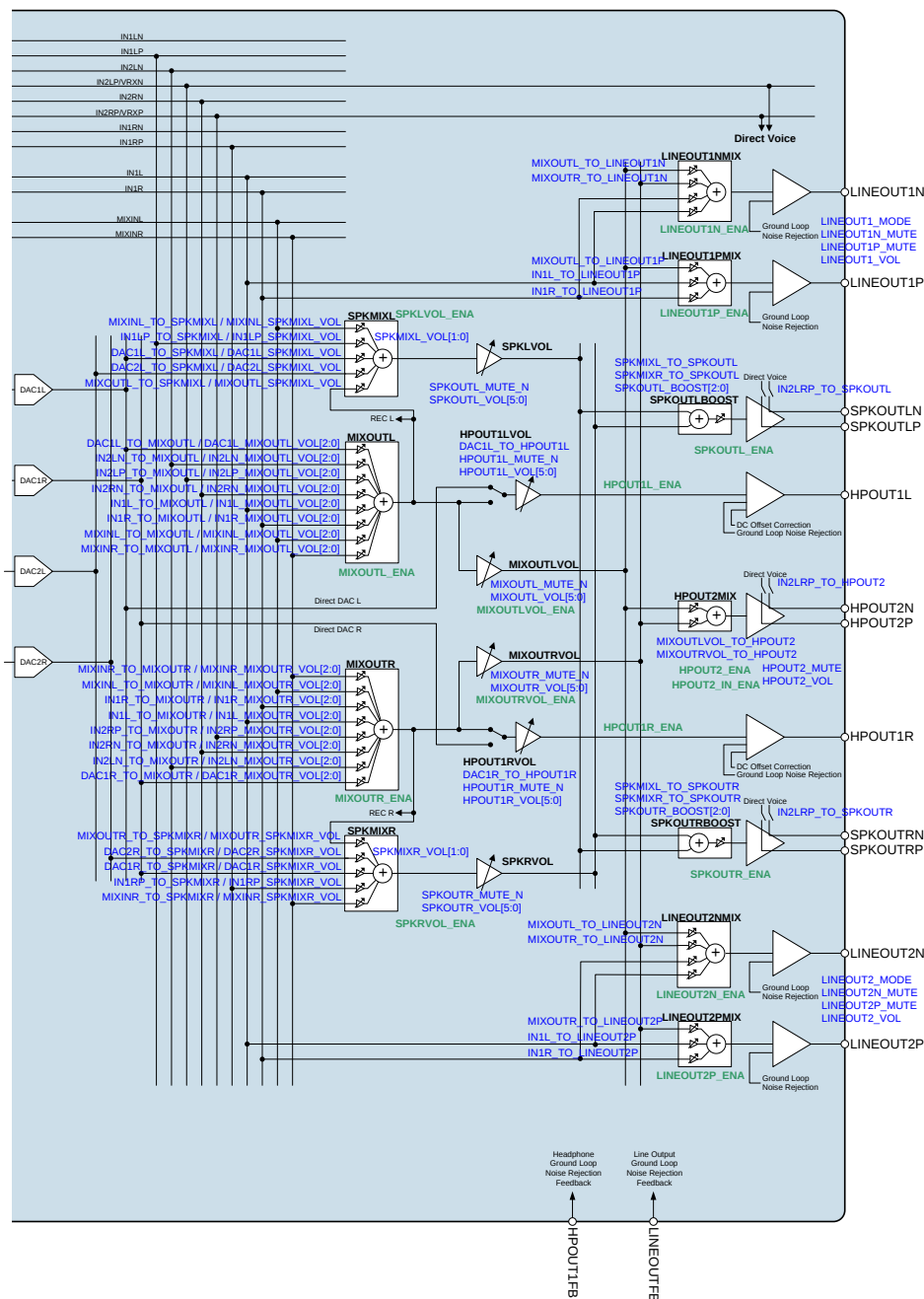
Figure 31 Control Registers for Output Signal Path
