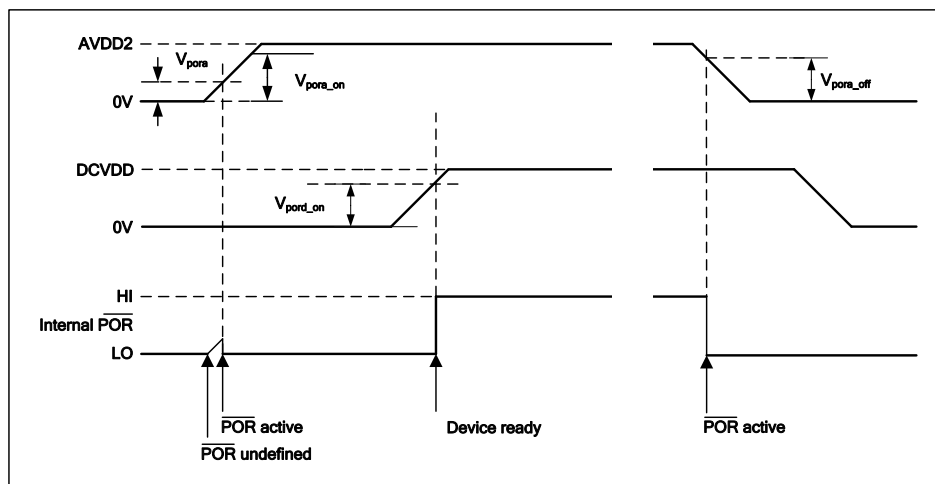
Figure 85 Power On Reset Timing – AVDD2 enabled/disabled first
