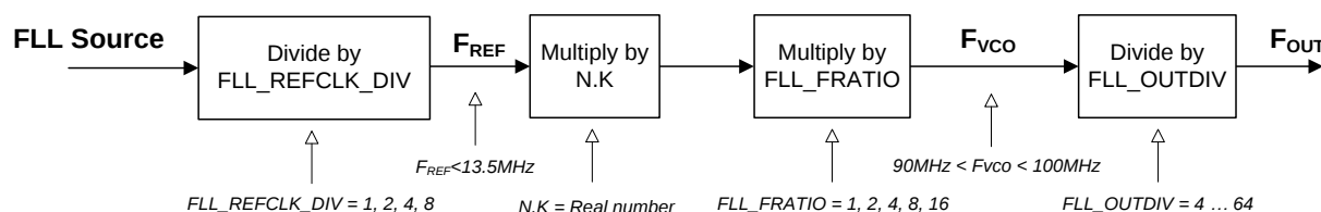
Figure 71 FLL Configuration
