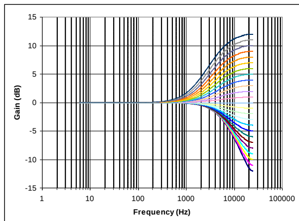
Figure 29 EQ Band 5 – High Freq Shelf Filter Response
