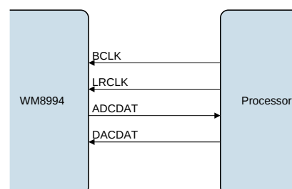
Figure 46 Slave Mode
