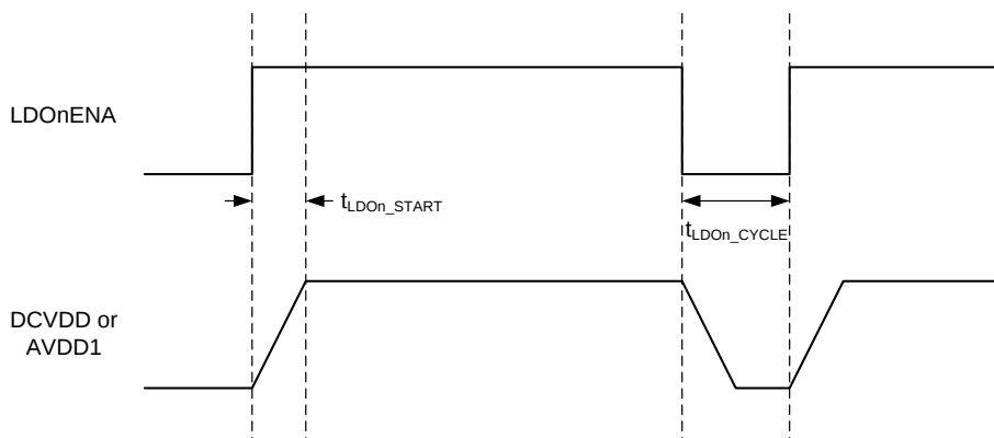
Figure 84 LDO Enable/Disable Timing Diagram
