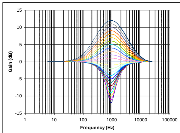
Figure 27 EQ Band 3 – Peak Filter Response
