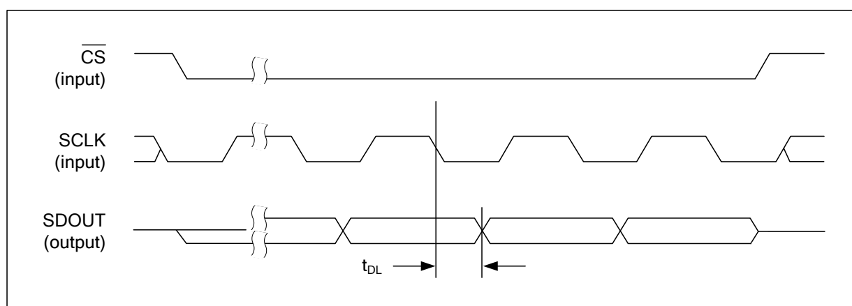
Figure 11 Control Interface Timing - 4-wire (SPI) Control Mode (Read Cycle)
