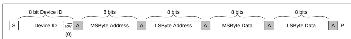
Figure 74 Single Register Write to Specified Address
