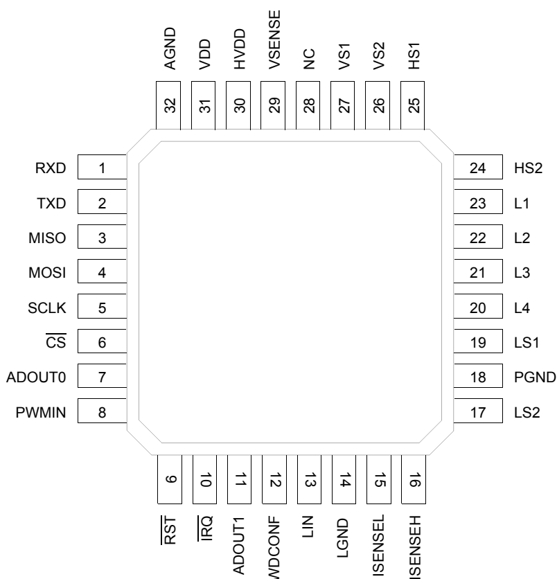
Figure 3. 33912 Pin Connections
