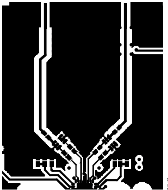
Figure 85. AD8364_EVAL-2140 Evaluation Board RF Area Layout
