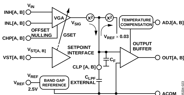
Figure 51. Single-Channel Details
