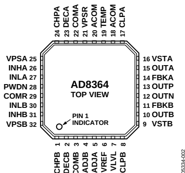
Figure 2. Pin Configuration
