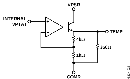
Figure 53. TEMP Interface Simplified Schematic
