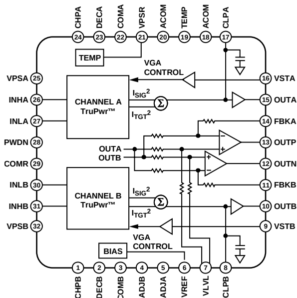
Figure 50. Block Diagram
