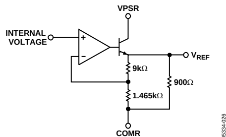
Figure 54. VREF Interface Simplified Schematic
