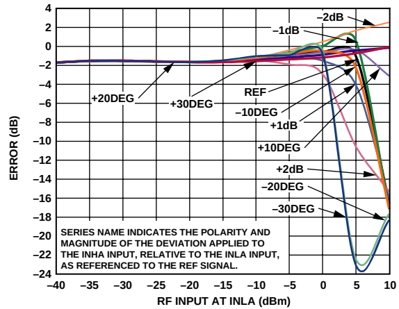
Figure 32. Log Conformance vs. Input Amplitude at Various Amplitude and Phase Balance Points, 2.500 GHz, Typical Device, ADJ[A, B] = 1.1 V, Sine Wave, Differential Drive
