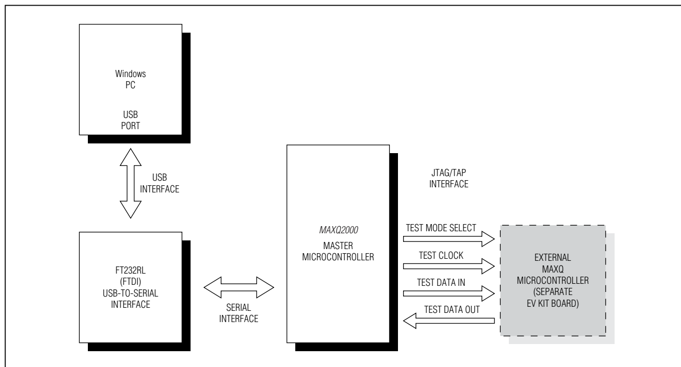
Figure 2. MAXQ USB-to-JTAG Communications Interface
