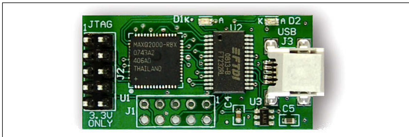
Figure 1. MAXQ USB-to-JTAG EV Kit Board
