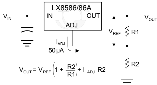
Figure 2 - Basic Adjustment Regulator
