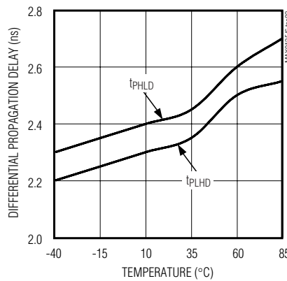
DIFFERENTIAL PROPAGATION DELAY vs. TEMPERATURE
