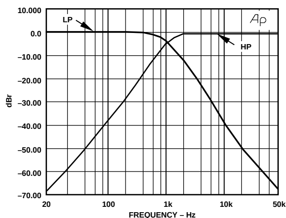
Figure 45. Relative Frequency Response of 2-Pole, 1 kHz Butterworth LP (Left) and HP (Right) Active Filters
