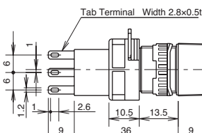
Solder/Tab Terminal
