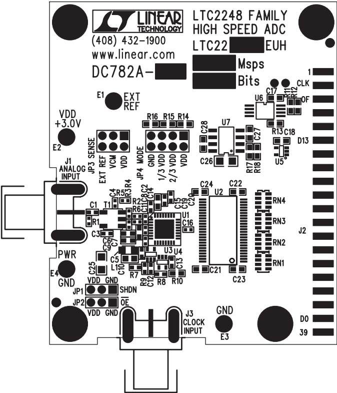
Silkscreen Top
