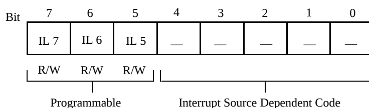
Figure 68. Interrupt Vector Low Register (IL: I/O Address = 33h)
