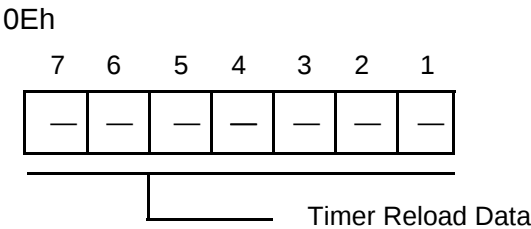
Figure 39. Timer Reload Register Low
