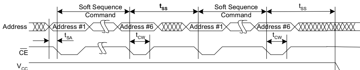
Figure 16. Soft Sequence Processing [30, 31]
