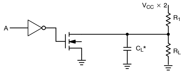
Figure 5. Test Circuit
