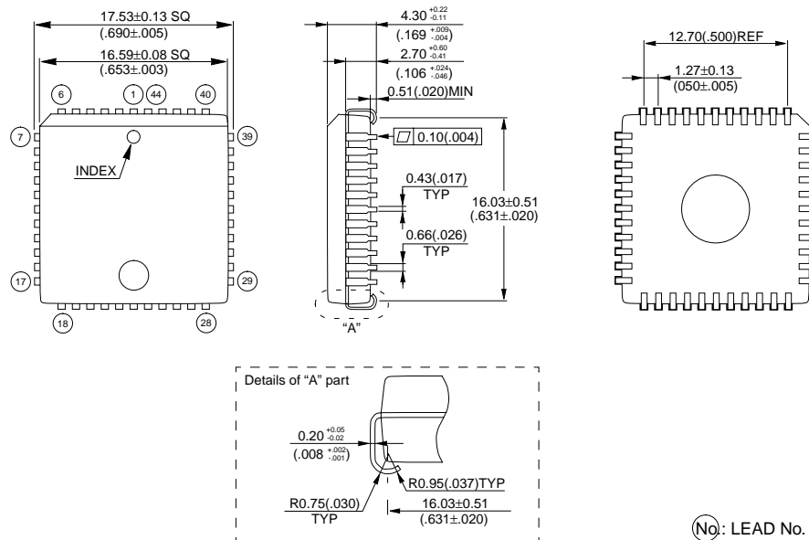
44-pin plastic QFJ (PLCC)
