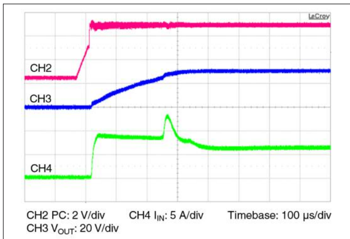
Figure 10 — Start up from application of PC; V_{IN} pre-applied C_{OUT} = 100\text{ }\mu\text{F}
