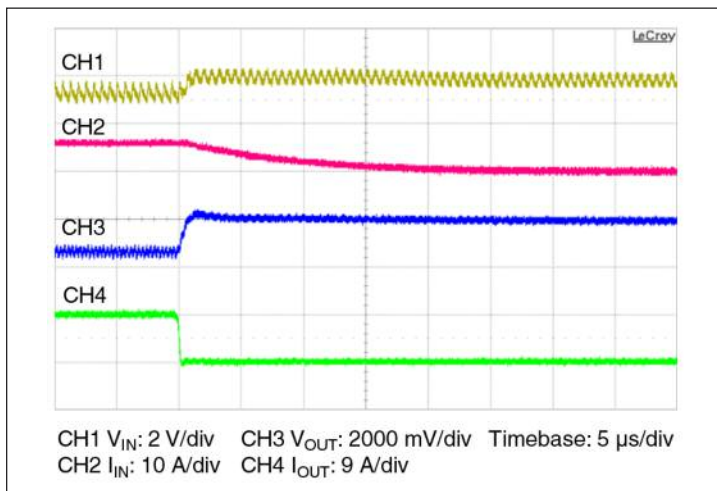
Figure 12 — 6.3 A–0 A transient response: C_{IN} = 330\text{ }\mu\text{F} , I_{IN} measured prior to C_{IN} , no external C_{OUT}
