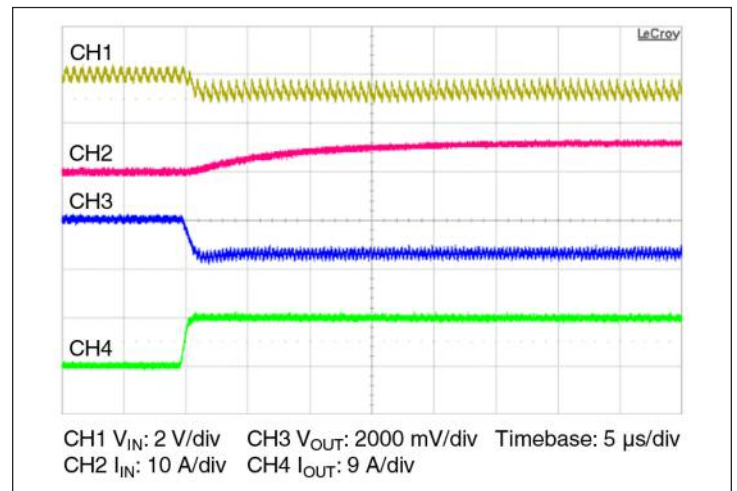
Figure 11 — 0 A–6.3 A transient response: C_{IN} = 330\text{ }\mu\text{F} , I_{IN} measured prior to C_{IN} , no external C_{OUT}
