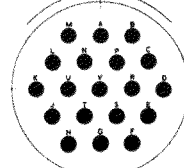
24-19 19 NO.12 CONTACTS
