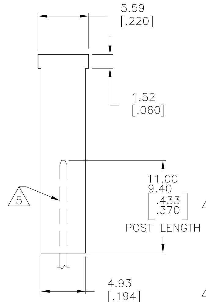
DETAIL X
