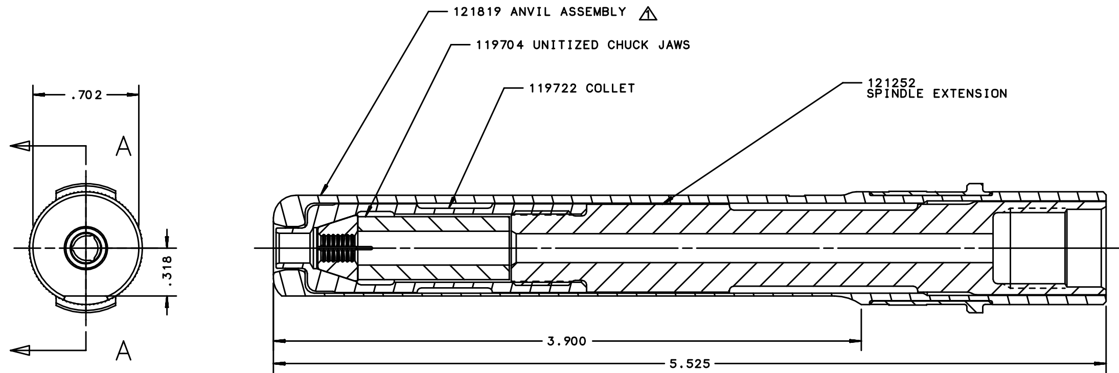
SECTION A—A
