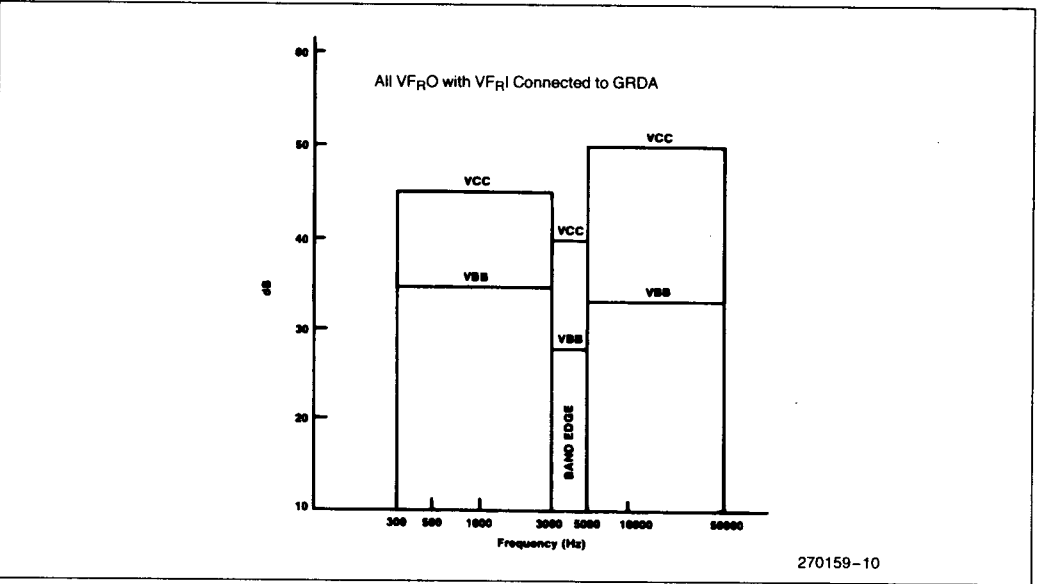
Figure 10. Receive Filter
