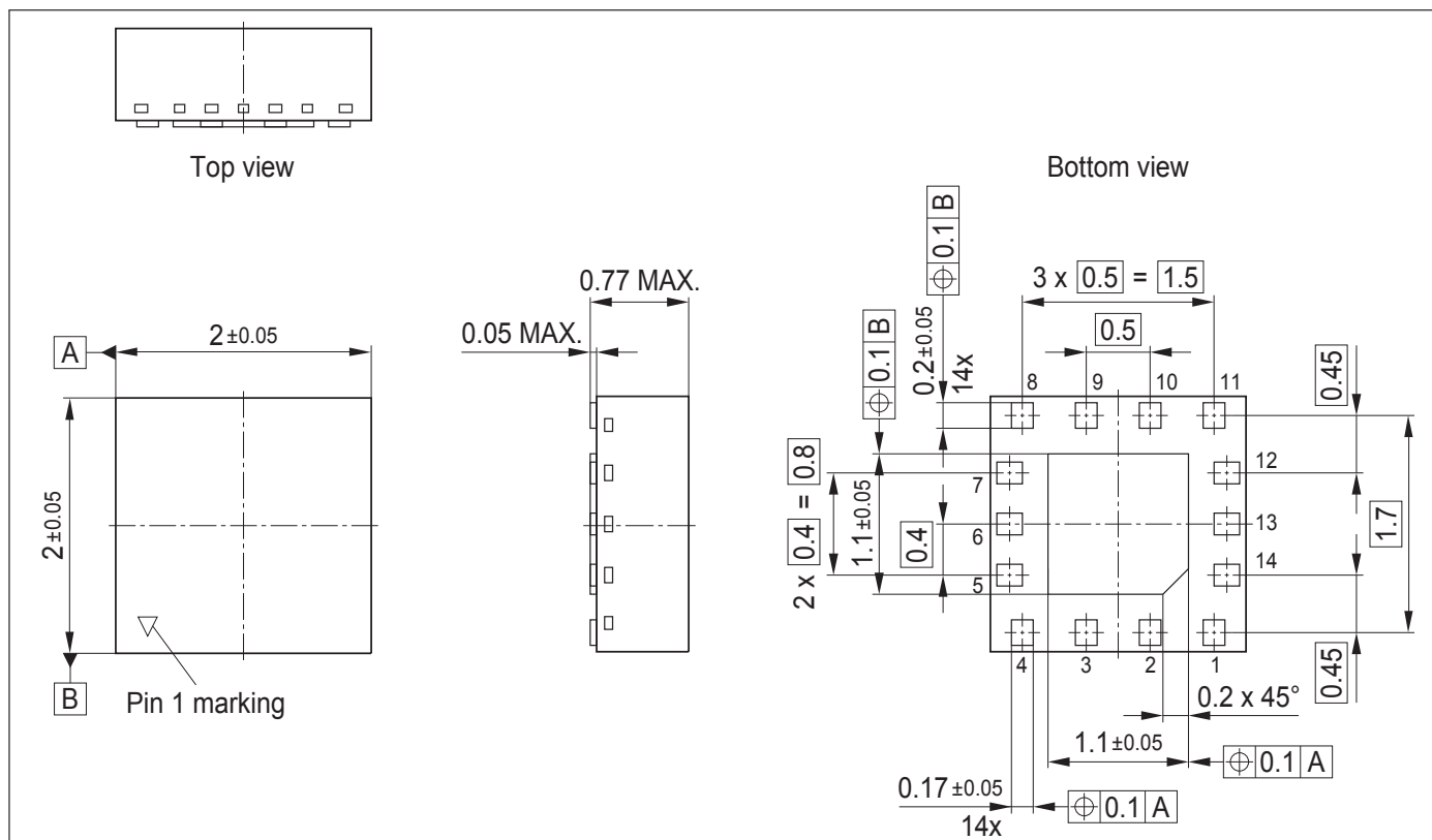
Figure 10: Package outline
