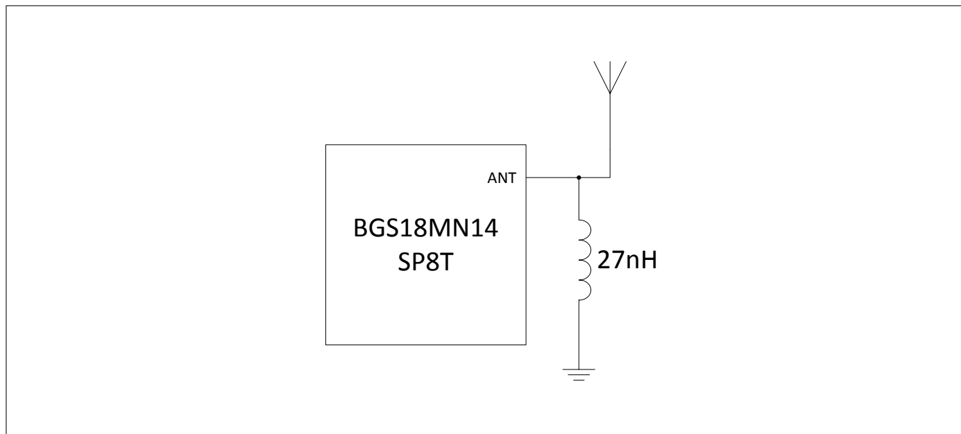
Figure 9: Application circuit
