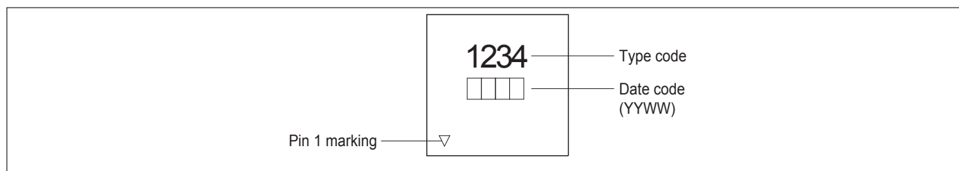
Figure 11: Marking
