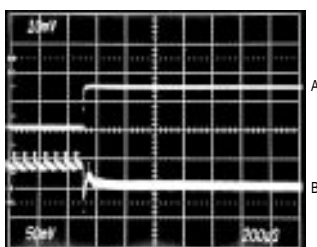
LOAD-TRANSIENT RESPONSE
