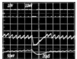
MODERATE-LOAD, IDLE-MODE WAVEFORMS
