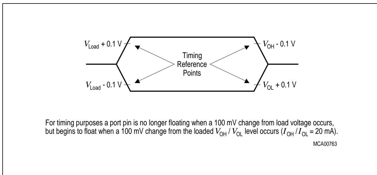
Figure 18 Float Waveforms
