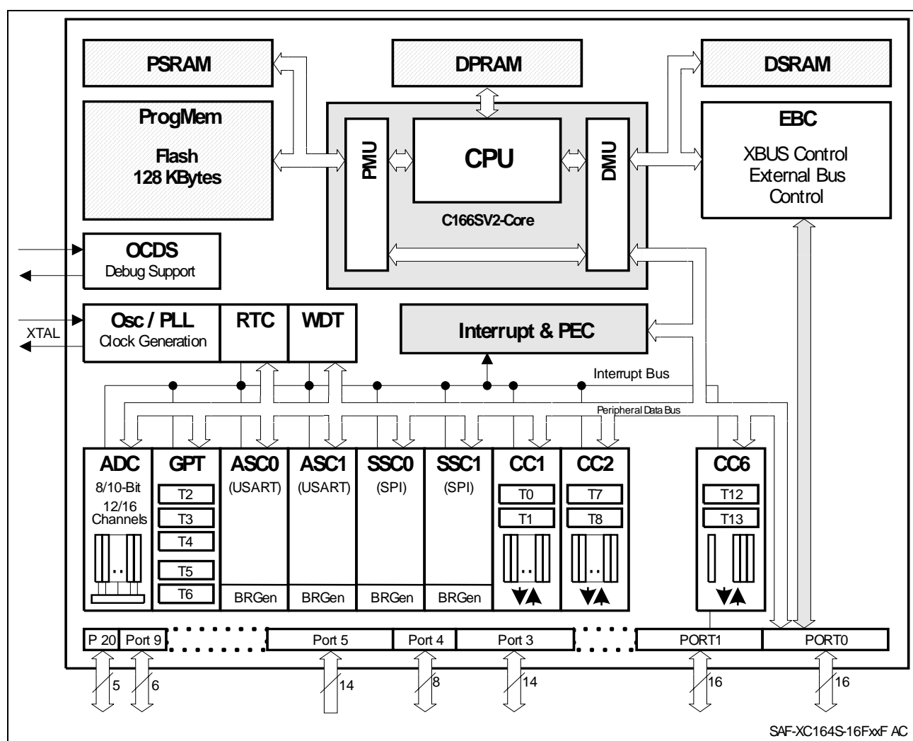
Figure 3 Block Diagram
