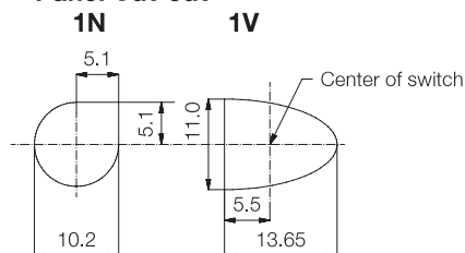
Panel Cut-out
