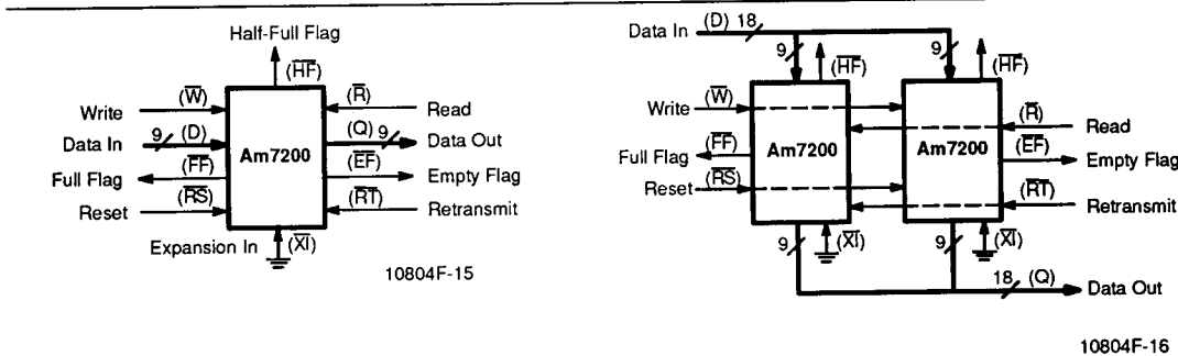
Figure 13. Width-Expansion to Form a 256 x 18 FIFO
