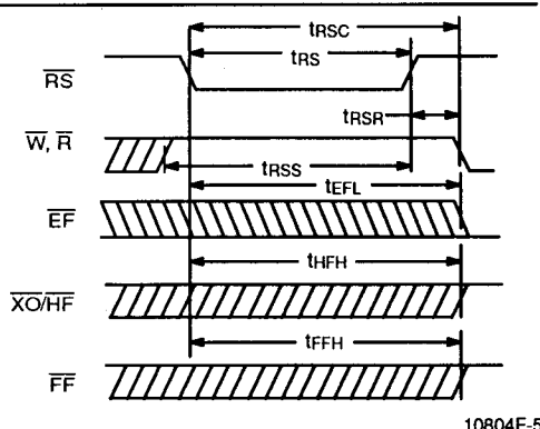
Figure 2. Reset Timing
