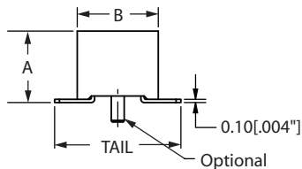
SFM210-, Dual Row, SMT Without Guide Posts (SM) or SMT With Guide Posts (SP)
