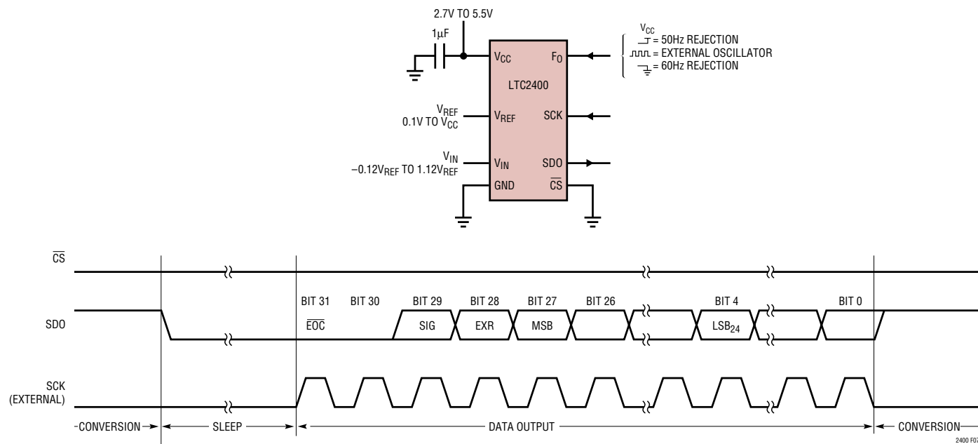
Figure 7. External Serial Clock, \overline{\text{CS}} = 0 Operation
