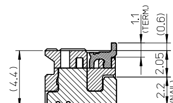
SECTION Z-Z
