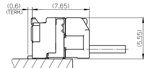
MATED CONNECTORS
