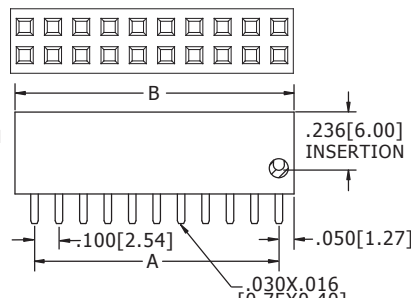
DUAL READOUT, STRAIGHT TAIL SHOWN
