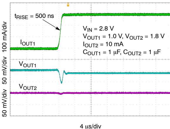
Figure 40. Load Transient Response – 1.0 V – Rising Edge, I_{OUT1} = 100 μA to 300 mA
