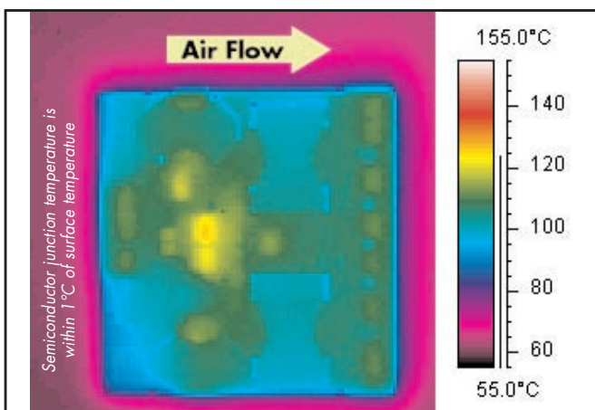
Figure 6: Thermal plot of converter at 26 amp load current with 55°C air flowing at the rate of 200 LFM. Air is flowing across the converter from input to output (nominal input voltage).
