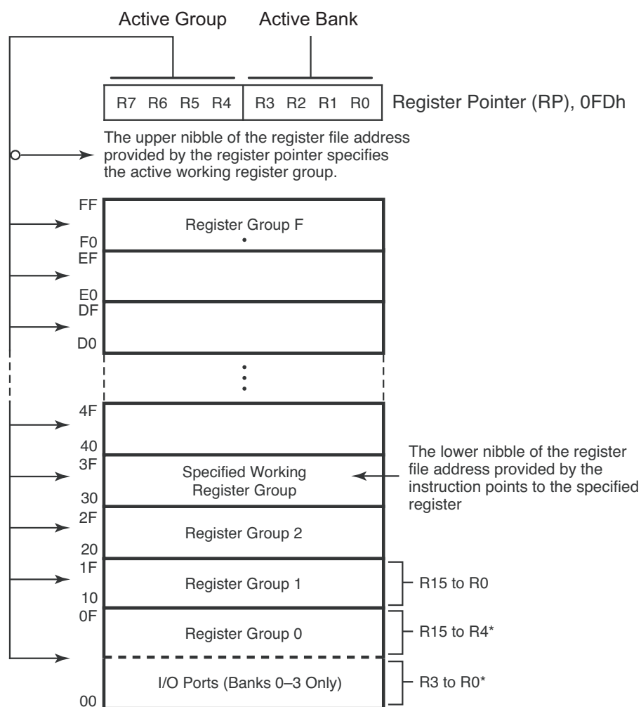
Figure 10. Register Pointer—Detail
