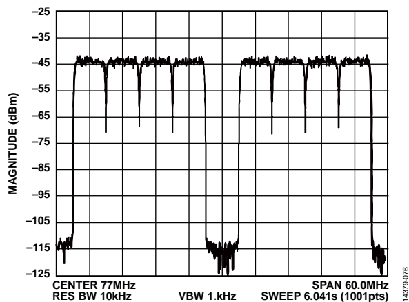
Figure 136. Gap Channel ACLR at 77 MHz
