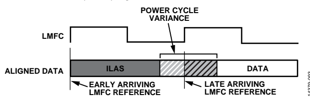
Figure 155. Link Delay &gt; LMFC Period Example
