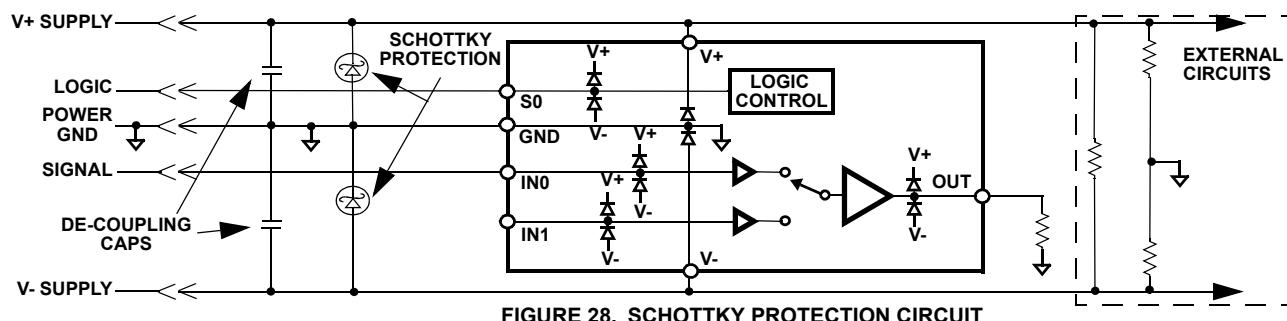
FIGURE 28. SCHOTTKY PROTECTION CIRCUIT
