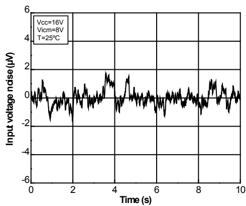
Figure 31. 0.1 to 10Hz noise
