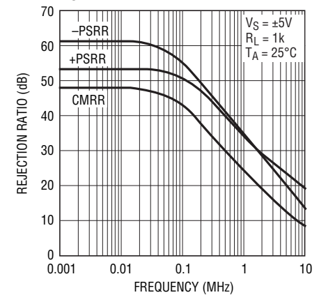
CMRR and PSRR vs Frequency ( I_S = 300μA per Amplifier)
