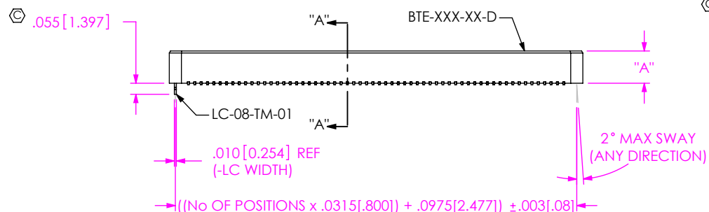
FIG 1 BTE-060-01-X-D-LC SHOWN
