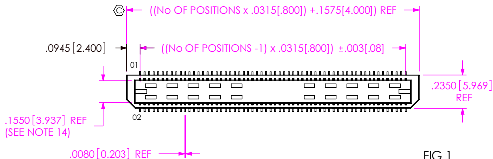
FIG 1 BTE-060-01-X-D-LC SHOWN
