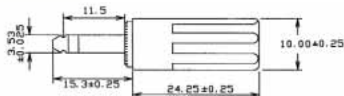
P5/P 3.5mm mono screened Jack Plug. Plated plastic body. Long Tip version for use with Far Eastern sockets P5P continental.
