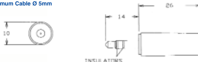
JPS-35 3.5mm stereo unscreened Jack Plug. Black plastic body only. JPS-35G Gold plated version.
