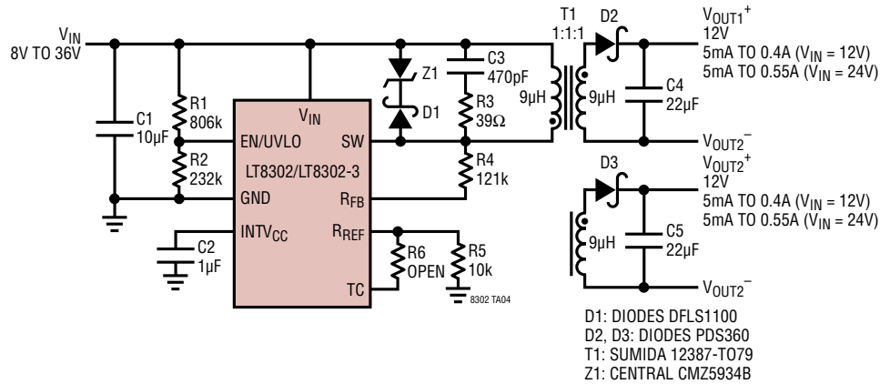
8V to 36V IN /±12V OUT Isolated Flyback Converter
