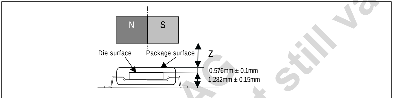
Figure 20: Vertical Placement of the Magnet
