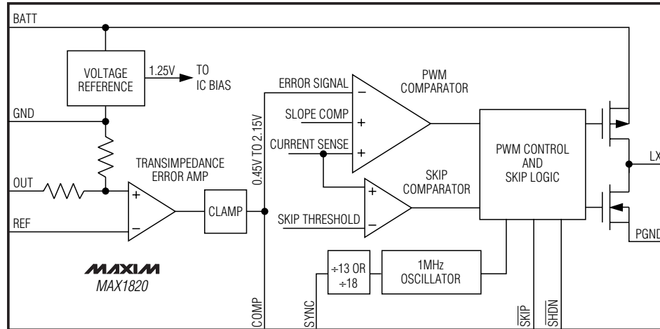
Figure 1. MAX1820 Simplified Functional Diagram (No SYNC for MAX1820Z)
