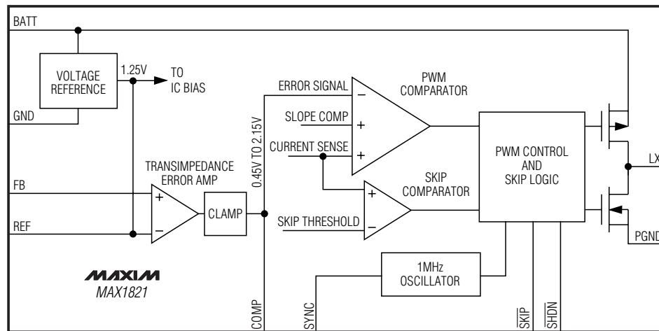
Figure 2. MAX1821 Simplified Functional Diagram (No SYNC for MAX1821)
