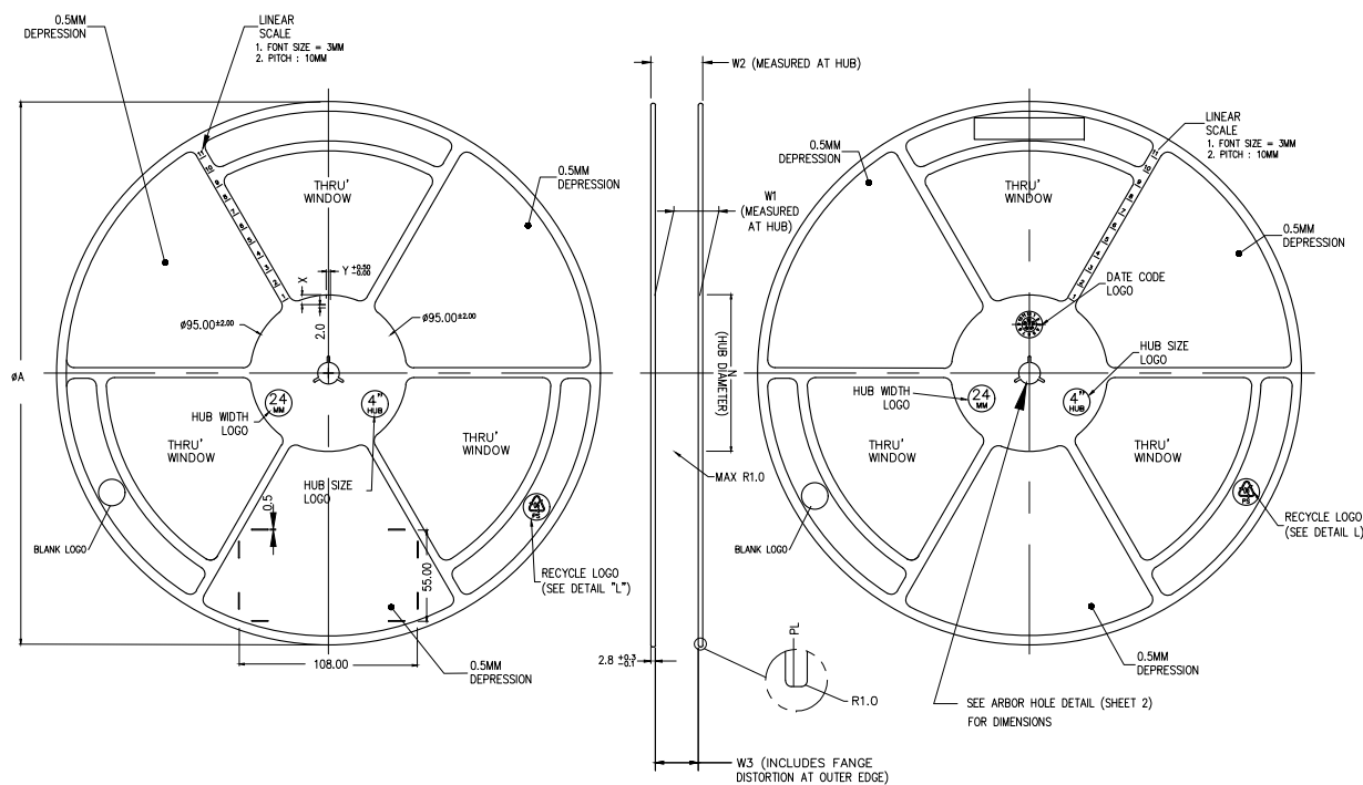
DIMENSIONS (MM)
