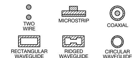
CROSS SECTIONAL CONFIGURATIONS OF VARIOUS TYPES OF GUIDING STRUCTURES
