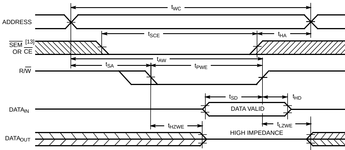
Write Cycle No. 2: \text{R}/\overline{\text{W}} Three-States Data I/Os (Either Port) [19, 21]
