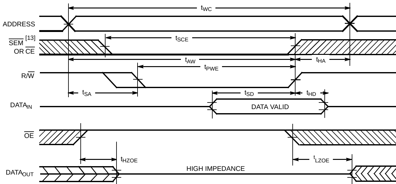
Write Cycle No. 2: \text{R}/\overline{\text{W}} Three-States Data I/Os (Either Port) [19, 21]
