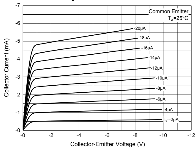
Fig. 7 - Static Characteristics
