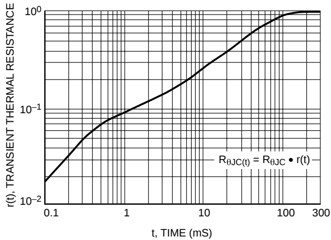
Figure 9. Thermal Response
