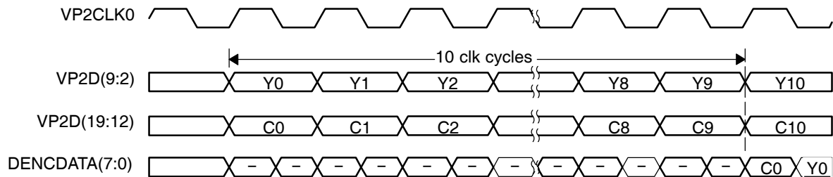
Figure 8. Video 16-bit, Double-clock-edge Output
