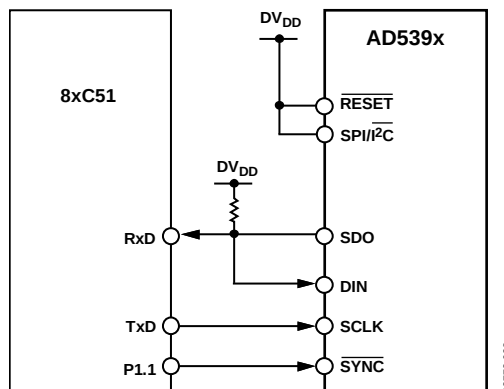
Figure 39. AD5390/AD5391/AD5392 to 8051 Interface
