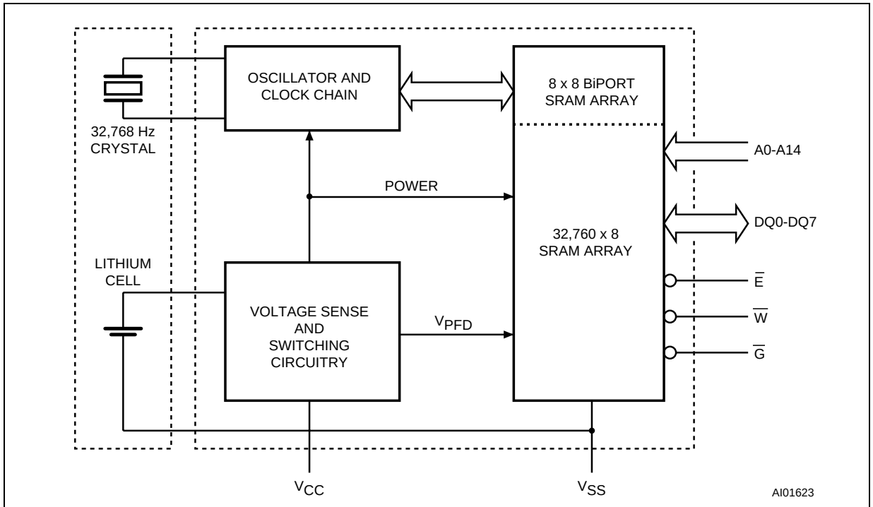
Figure 6. Block Diagram
