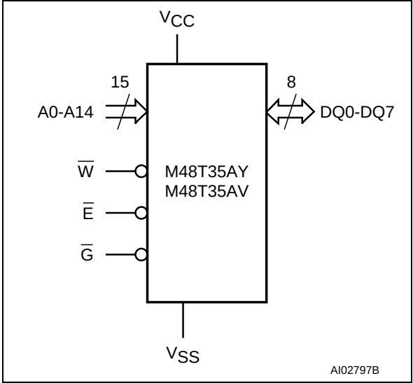
Figure 3. Logic Diagram
