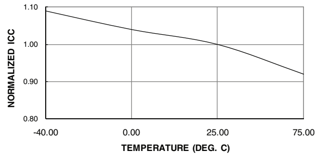
ATMEL ATF22LV10C NORMALIZED I_{CC} VS. TEMP.
